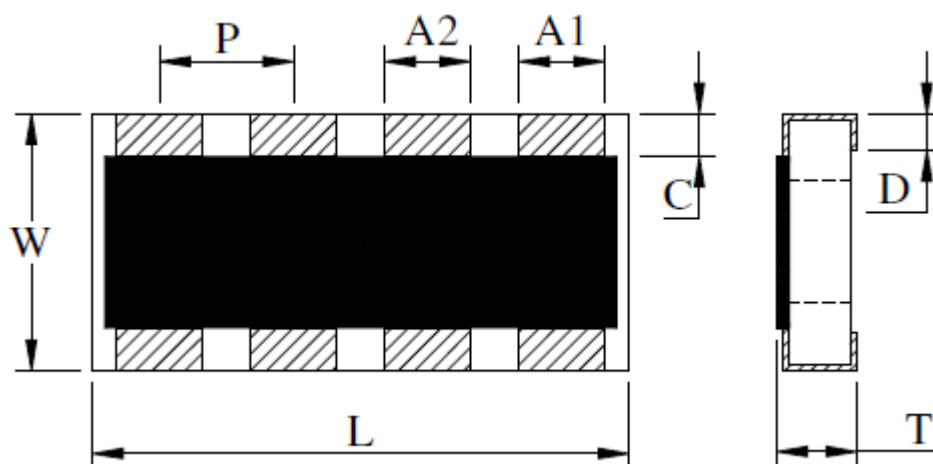
Fig 1. Outline of chip-R array WA02F
